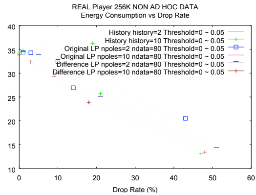
Fig 4.1. Drop Rate vs. Energy Metric Real Player, at 256 Kbps, results of history-based, linear prediction-based.
